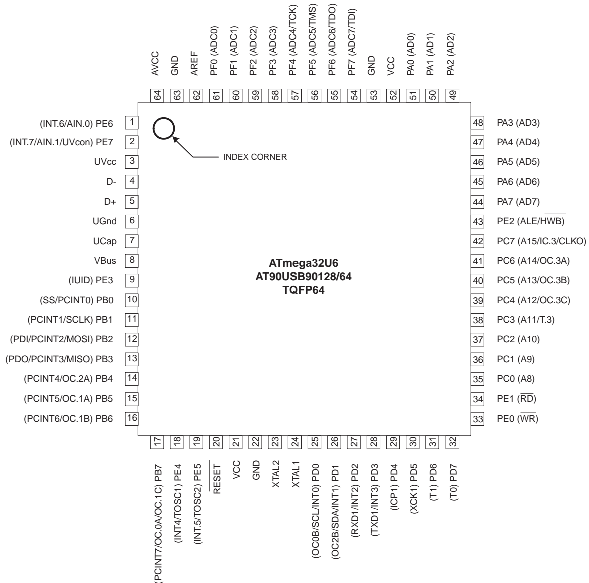
Figure 1-1. Pinout ATmega32U6/AT90USB64/128-TQFP
