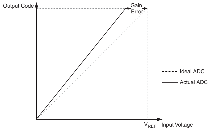
Figure 25-11. Gain Error
